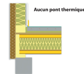
Plancher structure bois
